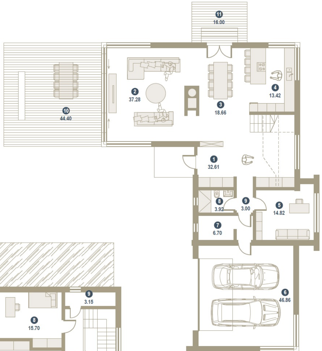
1ST FLOOR PLAN / m 2
